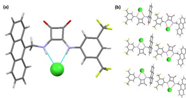
Figure 5. (a) Single crystal X-ray structure of the chloride complex of compound 1 and (b) self-assembly network formed between \text{Cl}^- and 1 . Counterions have been omitted for clarity.
